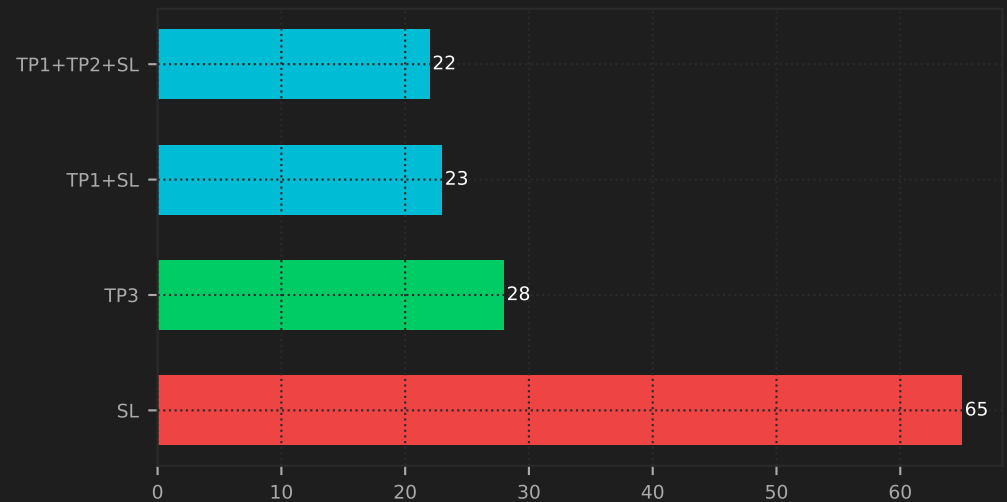
Exit Reasons
