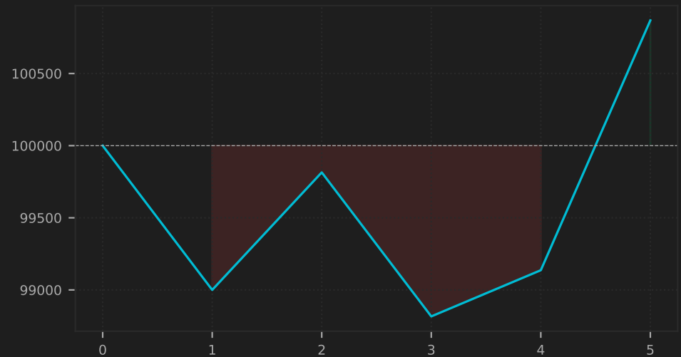
Equity Curve
